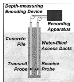
FIG. 3 Test Arrangement
