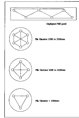
FIG. 4 Typical Access Duct Configurations
